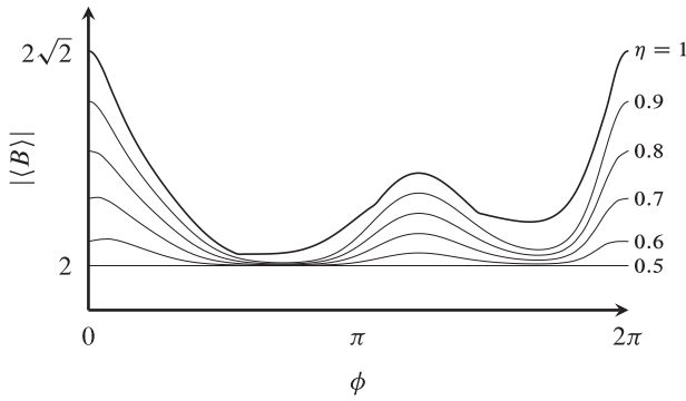
FIG. 3. Numerically optimized Bell-CHSH inequality test for |f\rangle as a function of the phase \phi . The Bell inequality can be violated as long as the detection efficiency \eta is larger than 0.5. For ideal photodetectors ( \eta = 1 ), the violation can be saturated, |\langle B \rangle| = 2\sqrt{2} at \phi = 0 ; the smallest violation is 2.044. Here, for simplicity, \phi = -\phi_c - \theta_c = \pi/2 - \theta_o .
