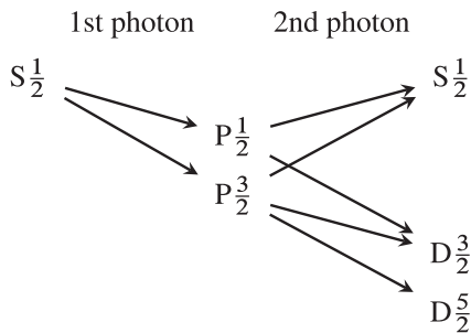
FIG. 4. Electric dipole selection rules between lj -states in one- and two-photon absorption. These two processes are distinguishable by the final orbital angular momenta, in particular, the separation into states with even (S, D) and those with odd parity (P).
