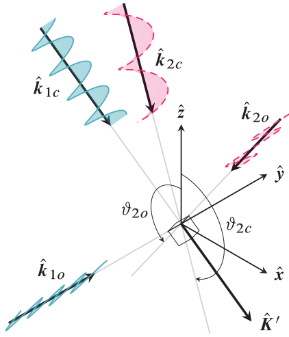
FIG. 2. Sample scattering geometry with incident light wavevectors \hat{k}_{1o} = \hat{y} , \hat{k}_{2o} with projection \hat{k}_{2o} \cdot \hat{z} = \cos \vartheta_{2o} = -\sqrt{2}/3 , \hat{k}_{1c} = \hat{K}' , and \hat{k}_{2c} with \cos \vartheta_{2c} = -2\sqrt{2}/3 . The emitted photoelectron is detected in the direction \hat{K}' . The alkali atom is located at the origin. The polarization of the incoming radiation is indicated in color (shades of grey). The o configuration uses linear polarization, whereas the c setup employs elliptically polarized light.
