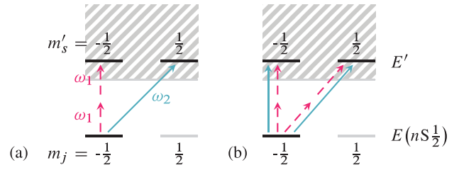
FIG. 1. Proposed coherent control interferometer (CCI). (a) In the open configuration o , single-photon ionization (solid blue) only undergoes a \sigma -transition with |m_j - m'_s| = 1 , whereas two-photon ionization (dashed red) leaves the electron spin unchanged. The processes are distinguishable from one another due to their different outcomes. (b) This is not the case in the closed setup c , for which the transition amplitudes between all spin combinations are nonzero.
