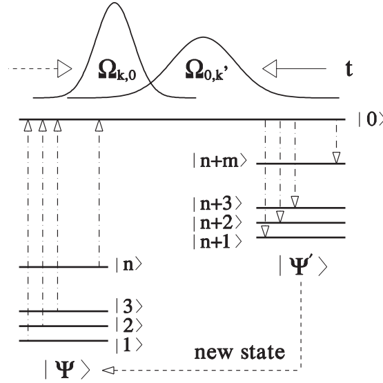
Figure 43. A transfer scheme between the states |\Psi\rangle \rightarrow |0\rangle \rightarrow |\Psi^e\rangle . The first (dump) laser pulse, with Rabi frequencies \Omega_{0,k'}(t) , couples all the |k'\rangle final (empty) states to state |0\rangle , while the second (pump) pulse, with Rabi frequency \Omega_{k,0}(t) , couples state |0\rangle to the initial (populated) states |k\rangle . Taken from figure 1, [169].
