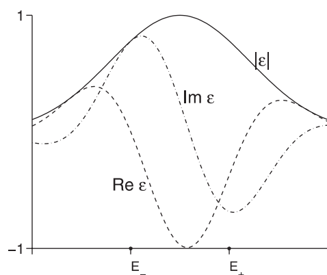
Figure 48. The light pulse (in frequency space) used to excite the Autler-Townes split |2P_0\rangle state from the ground 1S state to produce the optimal c_\alpha coefficients. This choice of coefficients is the one most effective in delaying the emission (in the absence of the interruptions) over the optimization time of 2.4 ns.
