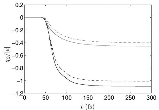
FIG. 1. Charge deposited in the left (solid lines) and right (broken lines) contacts during and after photoexcitation with pulse f4. Here, \hbar\omega = 1.3 eV, \phi_{2\omega} - 2\phi_\omega = 0 (black lines, flexible wire; gray lines, rigid case).
