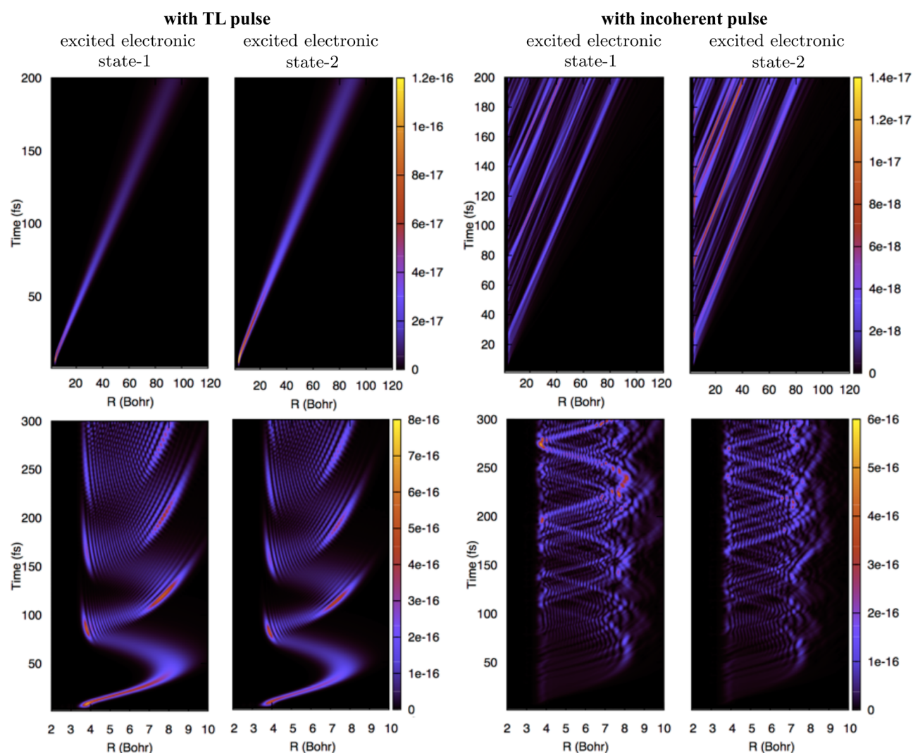
Figure 2. Spatiotemporal plots of the modulus-squared radial wave functions of the vibrational wave packets, u_x^{(1,2)}(R, t) . Top row is for case (A): purely repulsive excited state-1 and state-2 potentials. Bottom row is for case (B): bound Morse wells. The functional forms for both types of PES correspond to the first and third cases in Figure 3. Figures associated with the incoherent pulse refer to a single sample realization.
