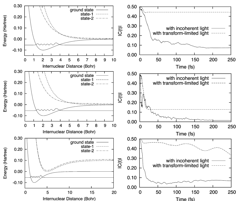
Figure 3. Left column: PES and the v = 5 vibrational wave function. Top panel: Repulsive PES of the form W_x^{(i)}(R) = W_0^{(i)} \exp[-(R - R_0^{(i)})/a^{(i)}] + W_\infty^{(i)} , i = 1, 2 ; where W_0^{(1)} = 0.1 hartree, R_0^{(1)} = 3.3 Bohr, a^{(1)} = 1.0 Bohr, W_\infty^{(1)} = 0 ; W_0^{(2)} = 0.1 hartree, R_0^{(2)} = 3.0 Bohr, a^{(2)} = 1.2 Bohr, W_\infty^{(2)} = 0.005 hartree. Middle panel: W_0^{(1)} = 0.1 hartree, R_0^{(1)} = 3.3 Bohr, a^{(1)} = 1.0 Bohr, W_\infty^{(1)} = 0 hartree; W_0^{(2)} = 0.1 hartree, R_0^{(2)} = 2.5 Bohr, a^{(2)} = 1.0 Bohr, W_\infty^{(2)} = 0.01 hartree. Bottom panel: W_x^{(i)}(R) = W_0^{(i)} [1 - e^{-(R - R_0^{(i)})/a^{(i)}}]^2 + W_\infty^{(i)} , i = 1, 2 ; where W_0^{(1)} = 0.1 hartree, R_0^{(1)} = 5.0 Bohr, a^{(1)} = 2.5 Bohr, W_\infty^{(1)} = 0 hartree; W_0^{(2)} = 0.1 hartree, R_0^{(2)} = 5.01 Bohr, a^{(2)} = 2.53 Bohr, W_\infty^{(2)} = 0.01 hartree. Right column: The absolute value of C(t) ; the normalized electronic coherence resulting from coherent and incoherent light excitation for the three different PES of the left column. The results for the incoherent light were averaged over a set of 10 random-jump realizations. (Additional realizations did not significantly alter the results.)
