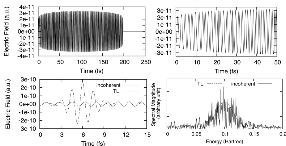
Figure 1. Upper left panel: a sample realization of incoherent light. Upper right panel: magnified view. The center wavelength is \sim 455 nm (corresponding to center energy of 0.1 hartree). The pulse has an envelope function of E_L(t) \approx [\sin(\pi t/200 \text{ fs})]^{0.1} for 0 < t < 200 fs and is zero elsewhere, chosen to simulate CW behavior with smooth turning on and off. The incoherent light is somewhat more coherent than solar radiation since we introduce, every 7 fs on the average, a random phase jump in the [-\pi, \pi] range, at a center frequency shift in the \pm 0.0175 hartree range. Lower left panel: A coherent pulse (denoted “TL” for transform limited) whose envelope is E_L(t) \approx \exp[-(t - 6 \text{ fs})^2/2(1.6 \text{ fs})^2] . A portion of the incoherent pulse from the upper panels is shown for comparison. Lower right panel: The frequency profile of the pulses of coherent and a single realization of incoherent light, demonstrating that both light sources share the same center frequency and the same spectral bandwidth.
